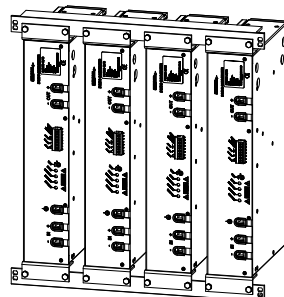
Figure 2. 19"-rack mounting
