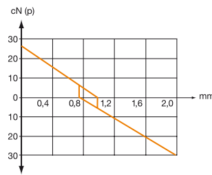
Contact force/travel
