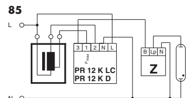
Electronic power reduction without control phase
