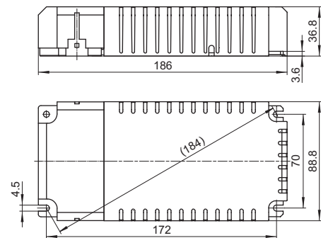
K31 with cord grip
