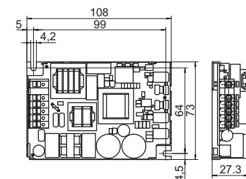
M3 built-in PCB
