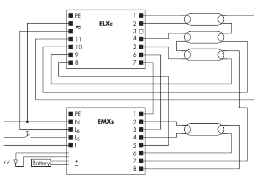
4-lamp operation - Warm start with electronic ballast ELXc
